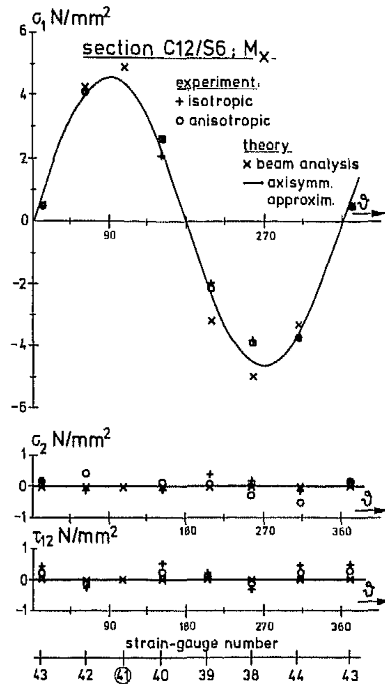
Fig. 15 Comparison of experimental and theoretical stresses in the principal material directions, shown as functions of \theta , in section C12, upon loading with a couple M_x' = 10,000 \text{ Nmm} .
