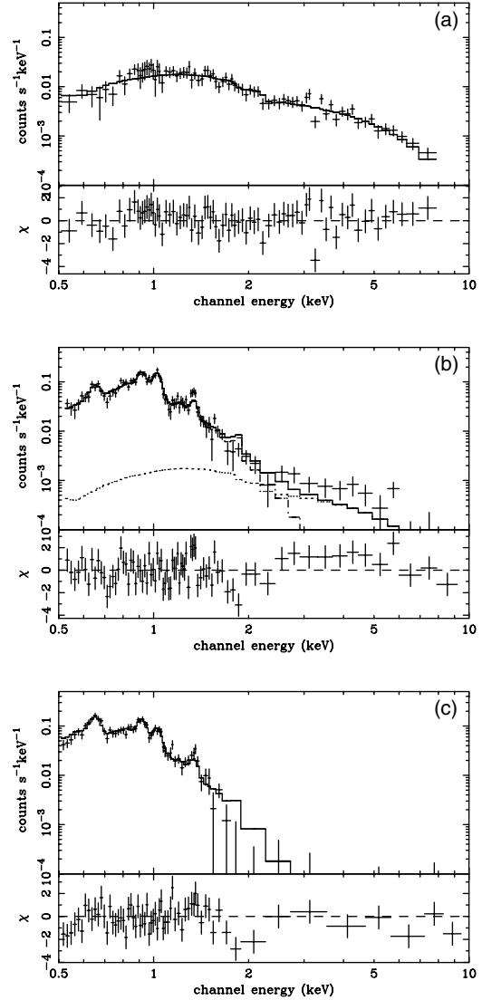
Fig. 4. Spectra of the Source 1 a) Head b) and Tail c) regions. Although we fitted the spectra of MOS 1+2 and pn CCDs simultaneously, only the MOS 1 data and results are shown for brevity. The best-fit models are shown with solid ( vps shock ) and dotted ( power-law ) lines. Lower panels in figures represent data residuals from the best-fit models.
