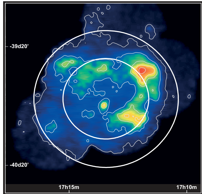
Fig. 1. X-ray image of RX J1713.7–3946 (colour scale and thin grey contour lines, 1–3 keV, from Uchiyama et al. 2002). The superimposed thick white contours indicate the 94% and 98% levels of the detection-efficiency weighted HESS exposure, given by the product of relative detection efficiency and the observation time. It can be seen that the relative gamma-ray detection efficiency between the centre region and the edges of the SNR differs only by \approx 5\% .
