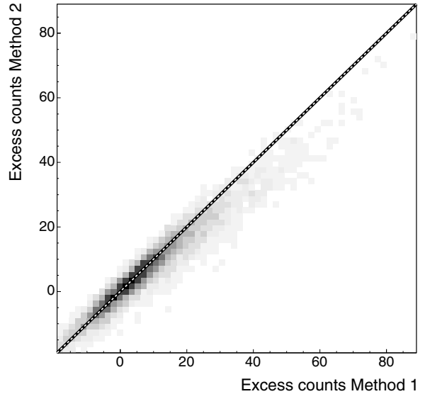
Fig. 6. Correlation between the standard calibration, event reconstruction, and background reduction method ( Method 1 ) and an alternative, completely independent approach ( Method 2 , see main text for more details). The black solid and white dashed lines run through the origin with a slope of 1. A linear correlation is clearly visible, deviations from the line originate from different cut efficiencies of the two methods.
