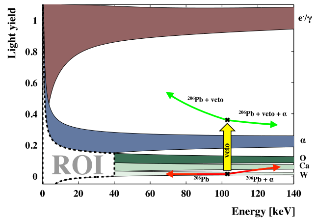
Fig. 1 Schematic plot of light yield vs. energy. Separate horizontal event bands arise: of beta/gamma events at LY \sim 1 (decreasing in LY at energies \lesssim 20 keV, see Eq. 2), of (degraded) alpha events at LY \sim 0.22 and of nuclear recoils off O, Ca and W at LY \lesssim 0.1 . Possible surface ^{206}\text{Pb} events appear at \sim 103 keV (at LY \sim 0.01 ) and – depending on their origin – above or below this energy (red arrows). If the corresponding alpha particles hit the scintillating housing, additional light is produced (veto) which shifts these events out of the nuclear-recoil bands (green arrows). The region of interest for dark matter search is indicated by a dashed black line. It includes the nuclear-recoil bands (O, Ca and W) and extends in energy from threshold (here: 0.6 keV) to 40 keV
