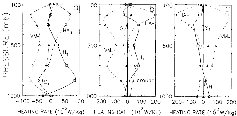
Figure 14. Vertical profiles of diabatic heating, H_T , ( \square — \square — \square — \square —); horizontal advection, HA_T , ( \circ — \circ — \circ — \circ —); vertical motion, VM_T , ( \triangle — \triangle — \triangle — \triangle —); and storage term, S_T , ( \blacktriangle — \blacktriangle — \blacktriangle — \blacktriangle —) for the composite Cyprus low at three selected gridpoints as follows: (a) 32.5^\circ\text{N} , 35^\circ\text{E} at the centre of the convective region in the cold front (point A in Fig. 8(e)); (b) 37.5^\circ\text{N} , 42.5^\circ\text{E} at the centre of the upward motion in the warm front (point B); (c) 35^\circ\text{N} , 22.5^\circ\text{E} at the centre of the downward motion in the wake of the cyclone (point C). Notice the different heating scales.
