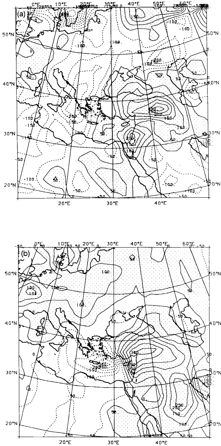
Figure 9. Distributions of vertically integrated: (a) diabolic heating, [H_T]_p ; (b) net condensation, [H_q]_p —for the composite Cyprus low, based on 1982–88 ECMWF analyses. Positive (solid) and negative (dashed) contours are plotted at intervals of 50 \text{ W m}^{-2} . Positive value regions are shaded.
