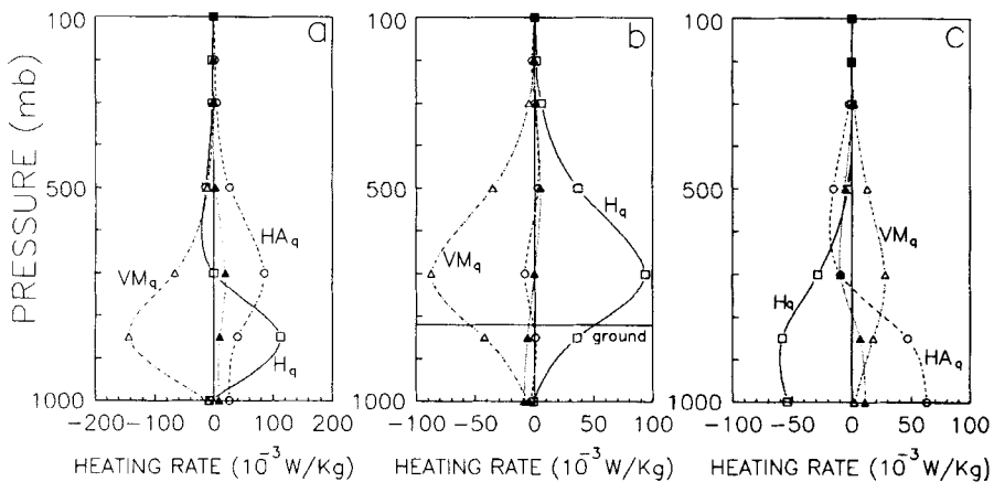
Figure 15. As in Fig. 14(a–c), but for the moisture budget terms.
