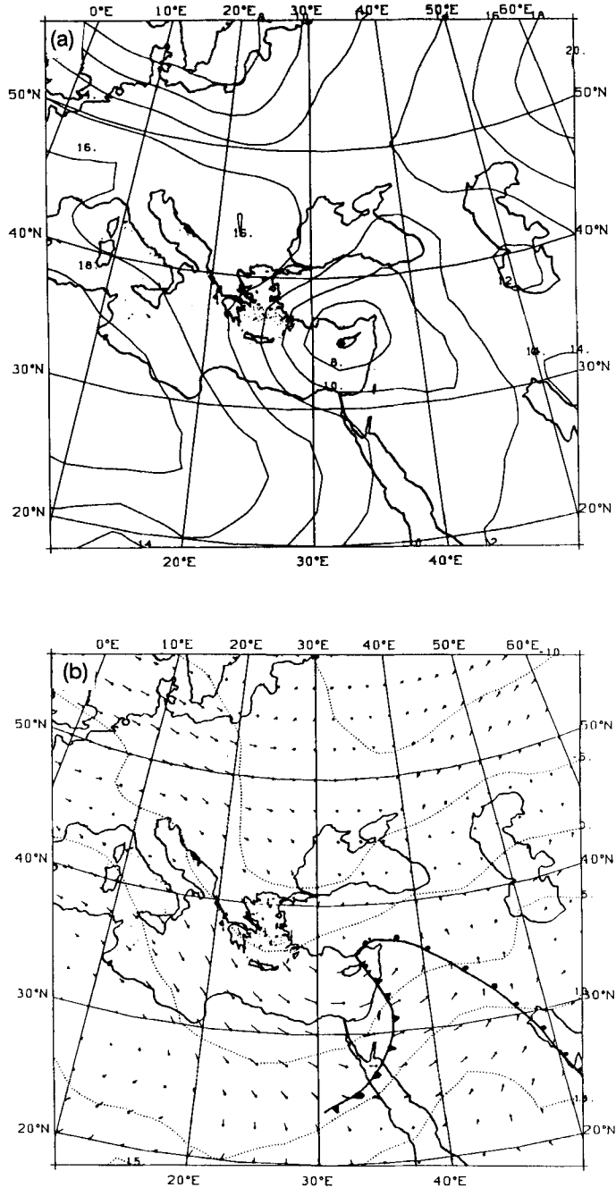
Figure 8. Main charts for the composite Cyprus low as follows: (a) 1000 hPa geopotential height (2 dam interval); (b) 850 hPa temperature (dotted, 5 K interval) and wind vector arrows representing 6-hour displacements; (c) 850 hPa rate of temperature advection with a 25 \times 10^{-3} \text{ W kg}^{-1} interval. Positive (solid) and negative (dashed) contours where positive-value regions are shaded; (d) 850 hPa geopotential height (solid, 3 dam interval) and relative humidity (dotted, 10% interval); (e) 500 hPa geopotential height (solid, 3 dam interval) and vertical p -velocity (dashed, 5 \times 10^{-2} \text{ Pa s}^{-1} interval, negative values shaded); (f) 200 hPa isotachs ( 10 \text{ m s}^{-1} interval; values exceeding 50 \text{ m s}^{-1} shaded) and 3-hour displacement wind arrows. The cold and warm fronts in (b) were plotted along the lines of maximum advection rate in (c).
