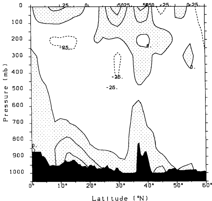
Figure 4. Vertical cross-section of the diabatic heating, \bar{H}_T , along 30°E longitude for an average winter (Dec.–Feb.) based on 1982–88 ECMWF data. Positive (solid) and negative (dashed) contours are at intervals of 25 \times 10^{-3} \text{ W kg}^{-1} . Positive-value regions are shaded. Topography is drawn in black at the bottom.
