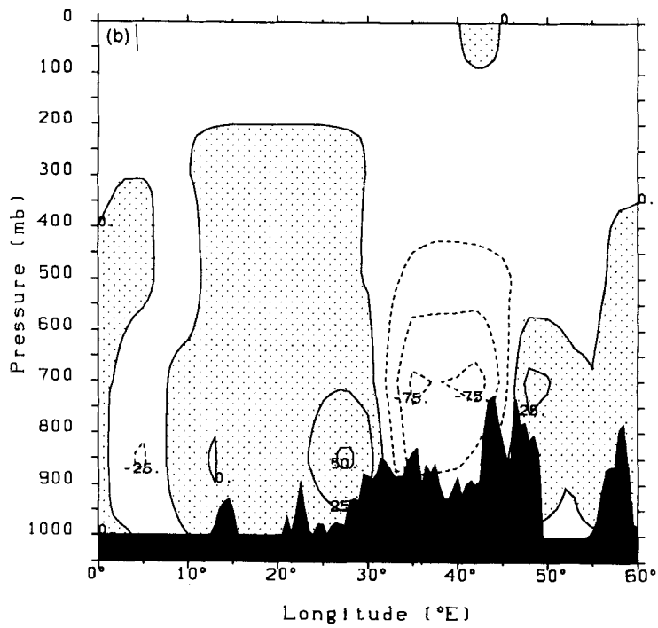
Figure 13. As in Fig. 12(a-d), but for the moisture budget terms.
