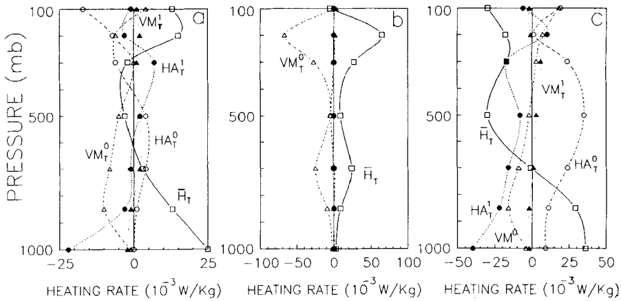
Figure 5. Vertical profiles of diabatic heating, \bar{H}_T , (—□—□—); steady horizontal advection, HA_T^0 , (○---○---); steady vertical motion, VM_T^0 , (△---△---); transient horizontal advection, HA_T^1 , (●---●---); transient vertical motion, VM_T^1 , (▲---▲---), for average winter (Dec.–Feb.) at three selected gridpoints as follows: (a) 35°N, 30°E, in the eastern Mediterranean; (b) 0°N, 20°E in the tropics; (c) 57.5°N, 5°E in the North Sea—based on 1982–88 ECMWF data. Notice the very different heating scales for the three regions. For further detail see Eq. (6) and text. Points A, B and C are as shown in Fig. 1(c).
