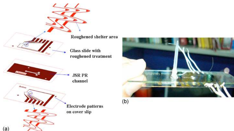
FIG. 1. (a) Chip design and construction. The electrode patterns of the bottom layer were fabricated on a thin cover slip and the electrode pattern of the top layer was fabricated on a treated glass slide. A roughened metal shelter was designed in front of the trapping electrode of the top layer that not only reduces the fluorescence noise but also enhances Raman signal. (b) Finished chip.
