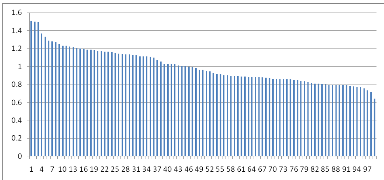
Figure 2. Distribution of scores using the multiplicative approach. Rank on horizontal axis.
