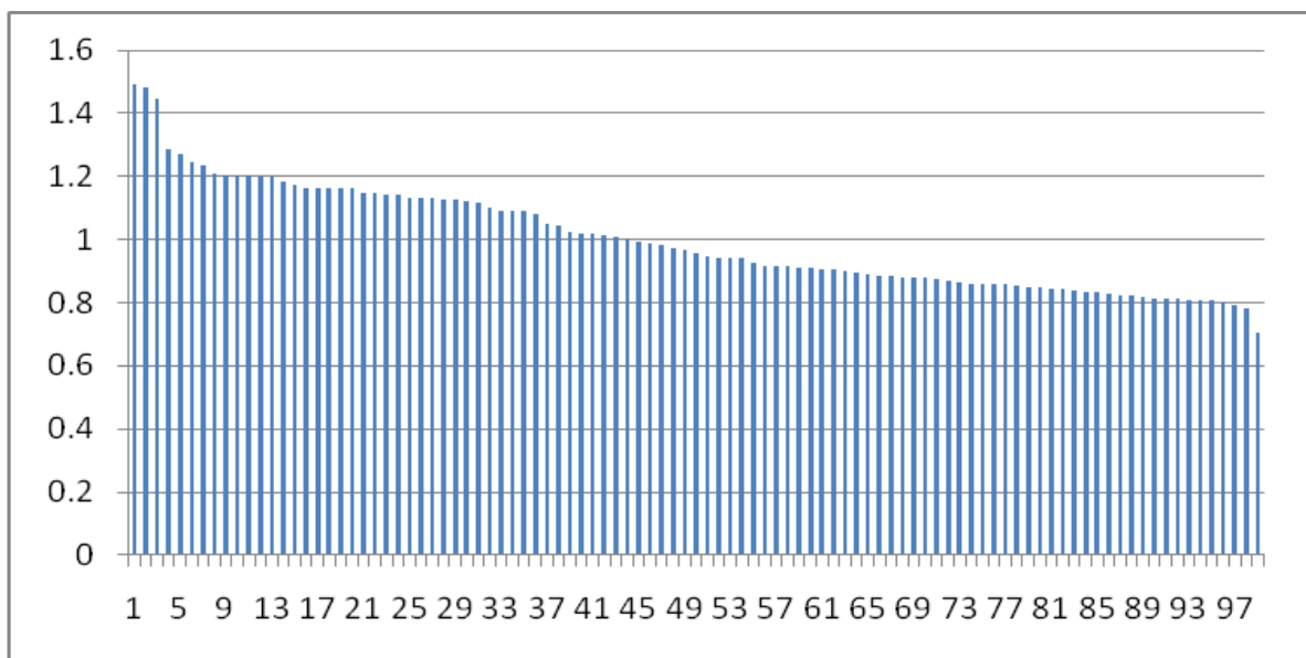
Figure 1. Distribution of scores using the additive approach. Rank on horizontal axis.
