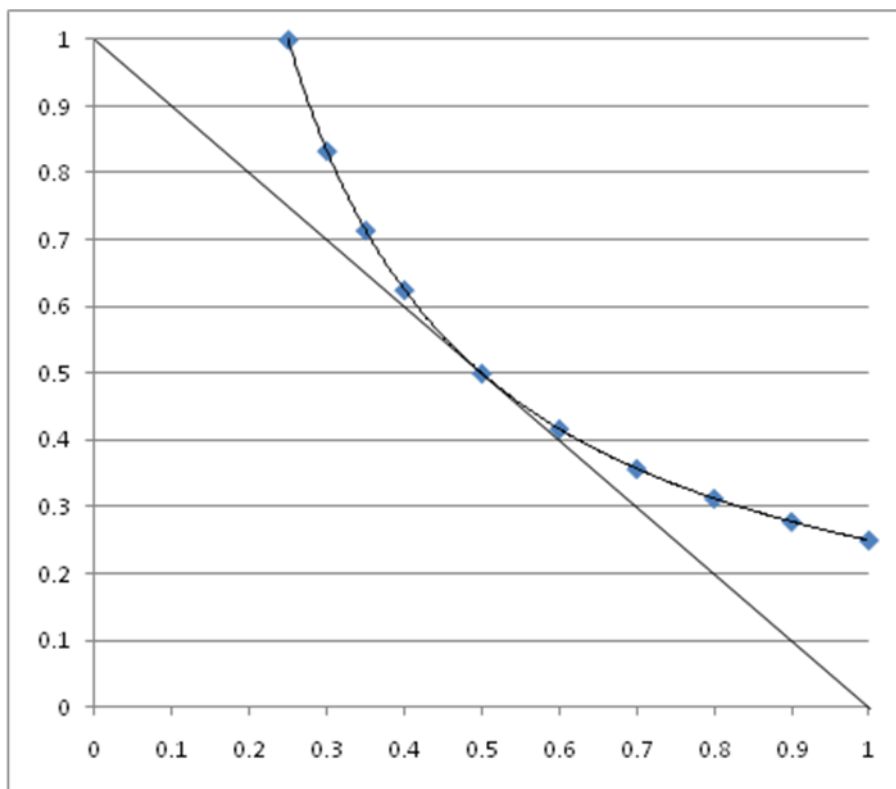
Figure 4. Contour lines for additive (straight) and multiplicative (curved) aggregations. Each point on the contour has the same score under its respective aggregation scheme.
