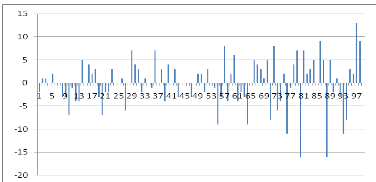
Figure 3. Difference in ranks between additive and multiplicative approaches (equal weights). A positive value implies that the institution was placed higher according to the multiplicative scheme. The horizontal axis shows the ordering as published in The Complete University Guide 2008 .
