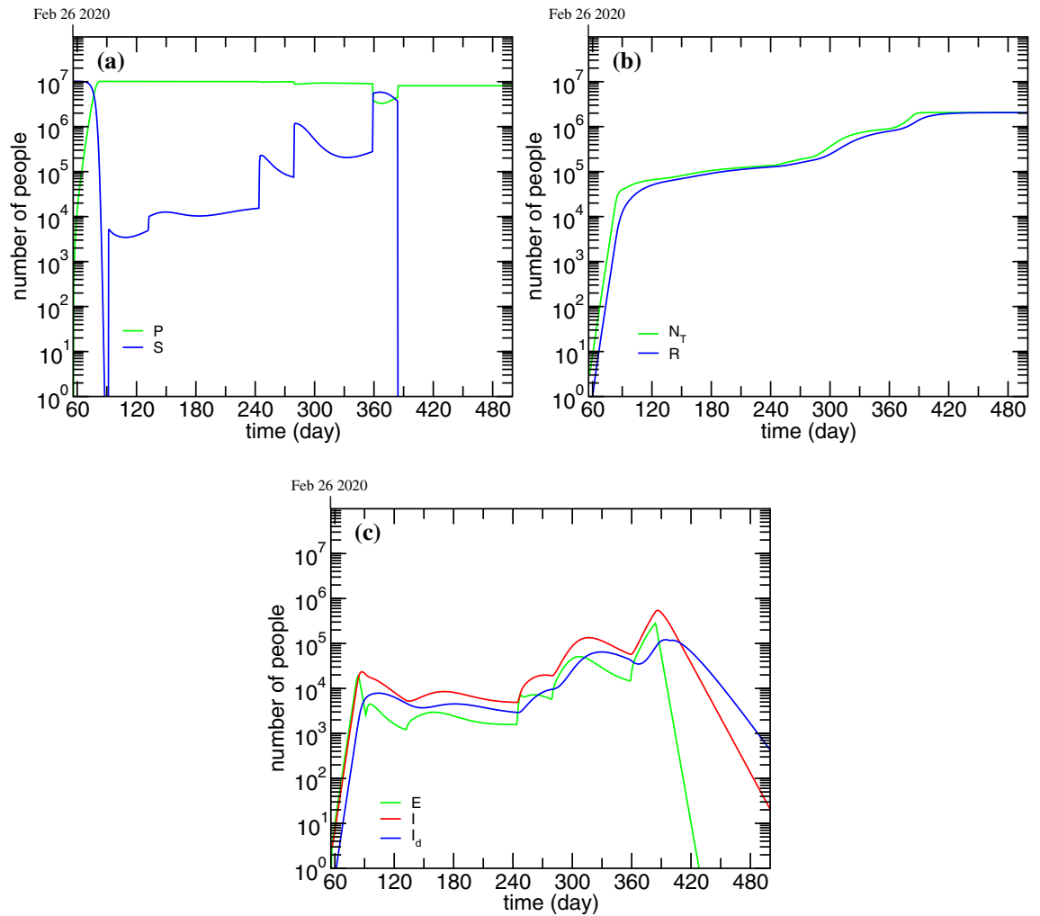
Figure 4. Time evolution of the total cases and of the modified PSEIRD(S) model compartments for which there is no available data or the data is not consistently reported: (a) P and S ; (b) N_T and R ; (c) E , I and I_d - c). The plots were obtained taking into account the same assumptions for the fixed parameters presented in Table 2 and the same optimized parameters presented in Table 2.
