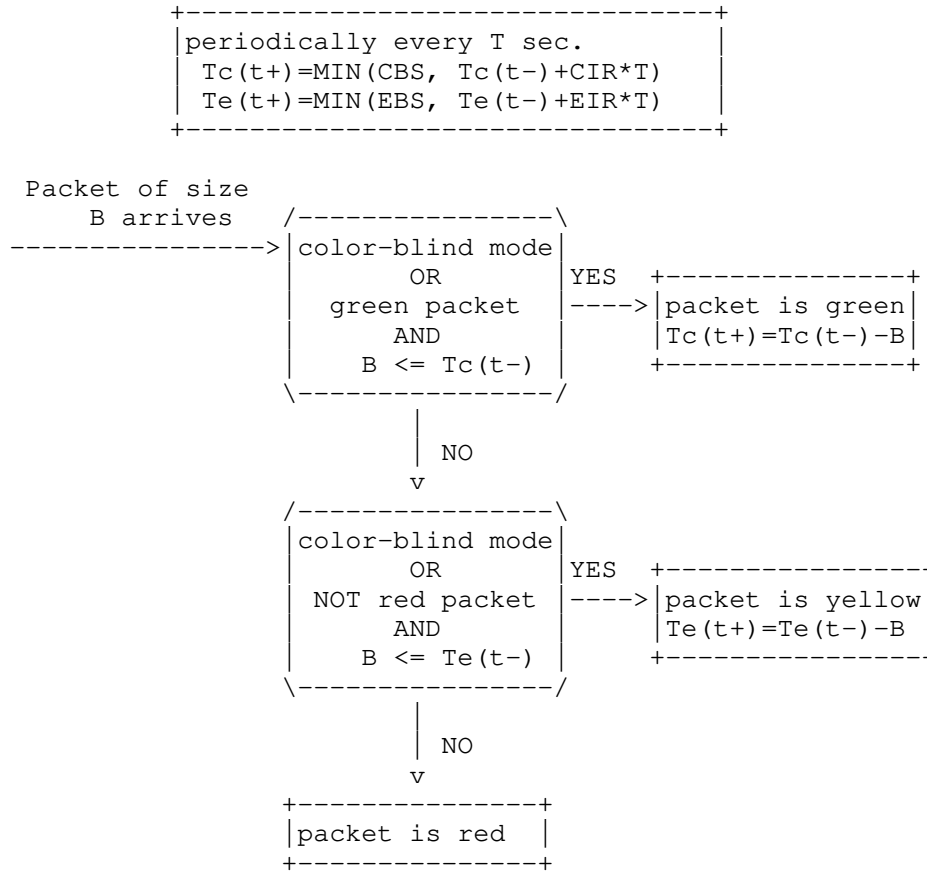
Figure 1: Traffic Metering/Marking Algorithm
