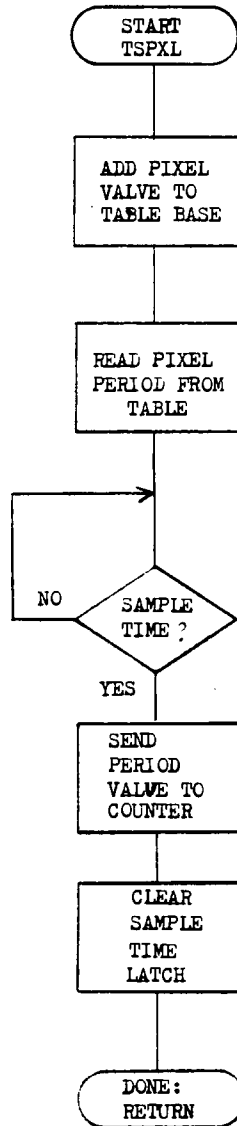
FIGURE 10 - SSTV TRANSMIT FLOW CHART
