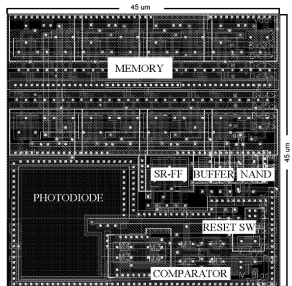
Fig. 7. Pixel layout, showing the main component parts.
