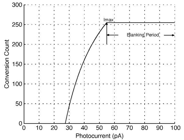
Fig. 3. Simulated ADC response using a fixed clock frequency and a blanking period set for a maximum photocurrent I_{\max} = 55 pA.
