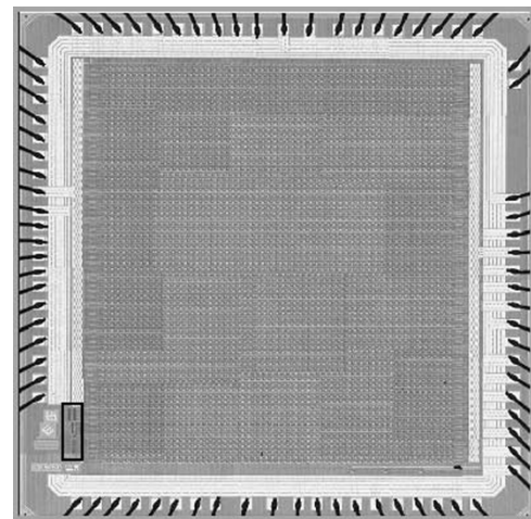
Fig. 8. Microphotograph of the 64 \times 64 pixel array, with the control circuit highlighted. The control circuits occupies less than 0.5% of the total chip area.
