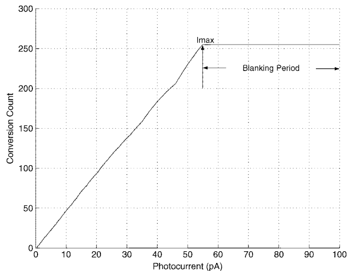
Fig. 4. ADC response using a variable frequency clock with a blanking period set for a maximum photocurrent I_{\max} = 55 pA.
