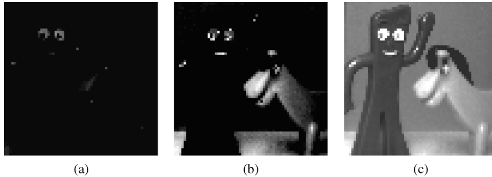
Fig. 13. Image capture operation under different settings, confirming earlier ADC simulations. (a) Image capture, fixed clock, no blanking. F_{Pr_i} = 3 kHz. (b) Image capture, fixed clock, with blanking. F_{Pr_i} = 3 kHz. (c) Image capture, variable clock, with blanking. F_{Pr_i} = 3 kHz.
