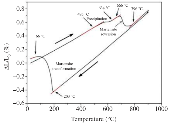
Figure 1. Dilatometric curve of heating and cooling for bar B, heating rate = 1 °C/s.
