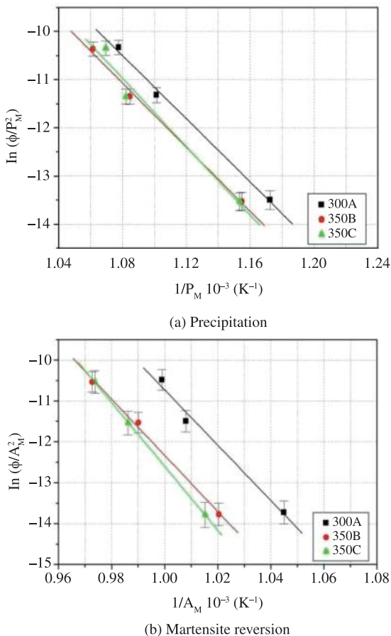
Figure 5. Method for the evaluation of the E values: (a) precipitation and (b) martensite reversion ( P_M is the temperature for which there is a maximum precipitation rate and A_M is the temperature for which there is a maximum martensite reversion rate, see Figure 4).
