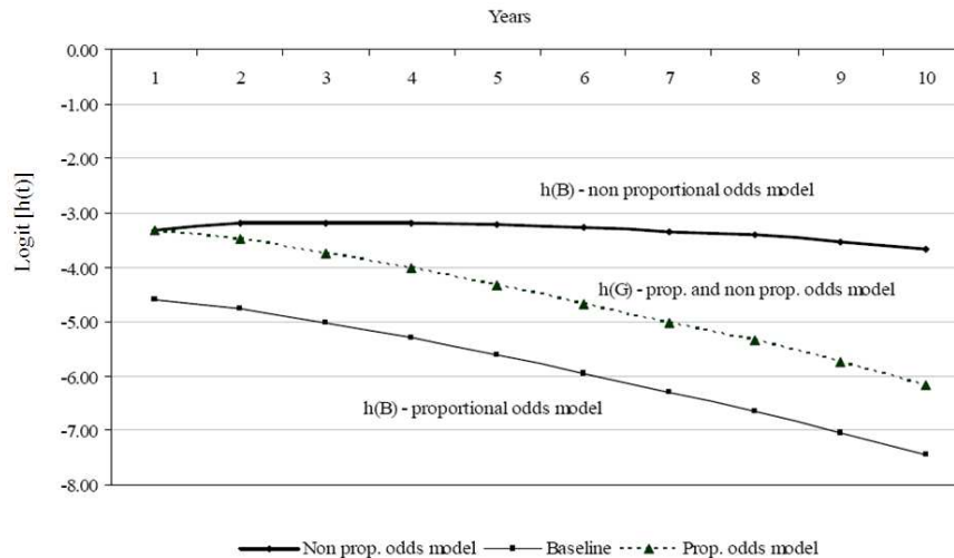
Fig. 4: Logit for “good borrowers” and “bad borrowers”, comparison of models
