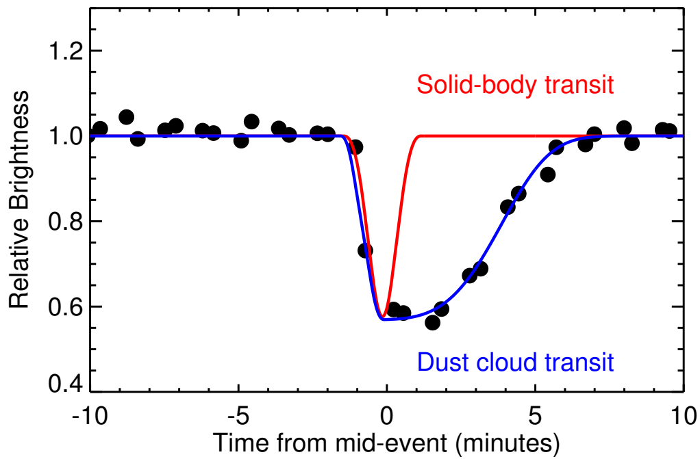
Figure S5: FLWO transits compared with a solid body transit model and a dusty tail transit model. The solid body model (shown in red) is calculated for a sub-Earth sized planet transiting a white dwarf with our stellar parameters in a 4.5 hour orbit, and has a much shorter duration than we see. The dust transit model (blue) simulates a dusty tail crossing over the star with optical depth \tau \propto \exp(-ax^4) , where a is a free parameter. The typical measurement uncertainties are smaller than the size of the symbols.
