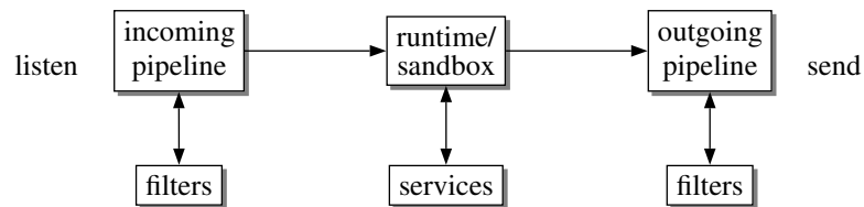
FIG. 3.1. The middleware runs a daemon which listens for incoming agents. Each agent is piped through several filters before it is admitted to the runtime system where it can access services by name. Agents can register and retrieve services by name (subject to access control). Before migration, each agent is piped through outgoing filters again.
