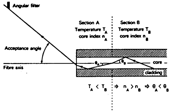
Fig. 4. Sensitivity of the mode-filter transmission to longitudinal variations of core index.
