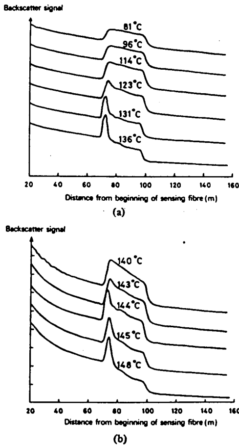
Fig. 15. Backscatter waveforms measured for large temperature differences on liquid-core fibers having low-loss claddings. (a) NA of launch fiber is 0.3. (b) NA of launch fiber is 0.2.
