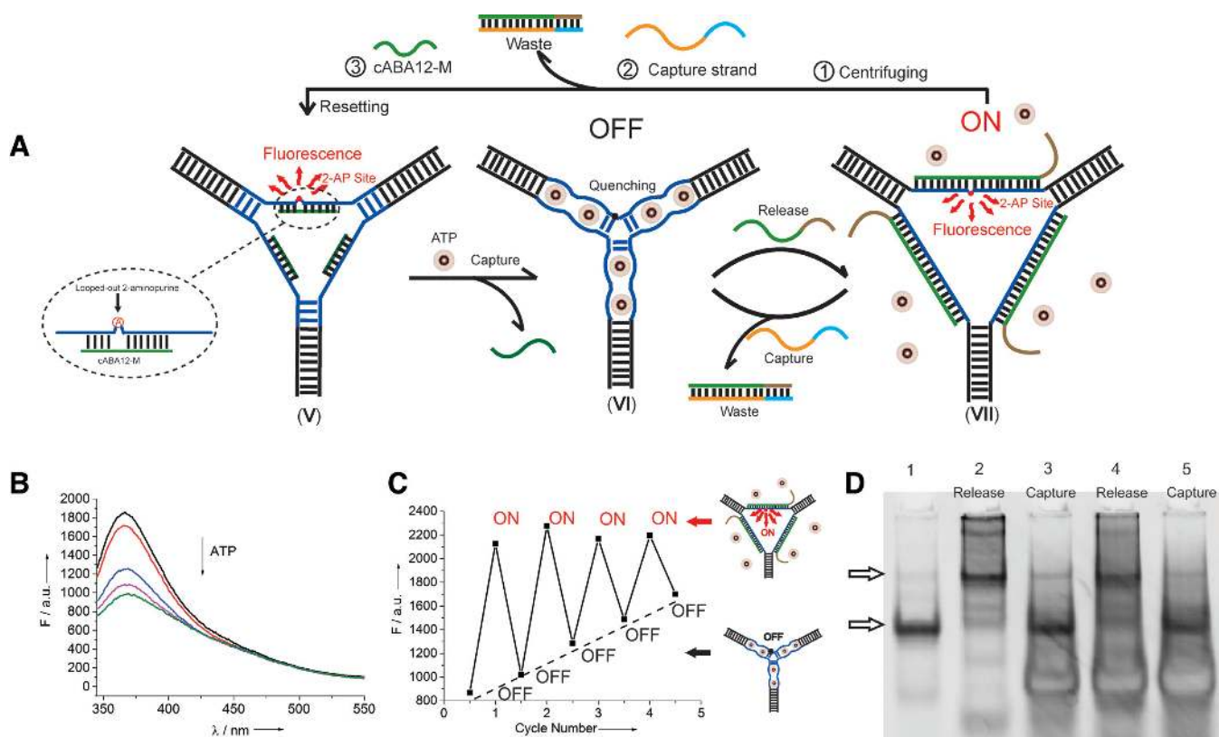
Figure 4. Generality of DNA switch-controlled reversible nanosensors. (A) Illustration of the working principle of the modified system: (V) Initial state of the modified ARTWN with a fluorescent 2-aminopurine bulge. (VI) ATP molecules intercalate into the embedded ATP aptamers, unwinding the 2-aminopurine bulge duplex with an obvious fluorescence decrease and placing the switch in the ‘OFF’ state. (VII) Upon the introduction of the release strands, the central ATP aptamers fully hybridize with them to form three rigid central duplexes, consequently releasing the ATP molecules and allowing the 2-aminopurine bulge to reappear, giving rise to a fluorescence increase. The switch is then in the ‘ON’ state. (B) Fluorescence emission spectra of 2-aminopurine with increasing concentrations of ATP (from top to bottom): 0, 200, 500, 1000, 2000 \mu\text{M} . (C) Switching processes of the DNA nanoswitch between ‘OFF’ and ‘ON’ state characterized by fluorescence emission spectra. (D) Switching performance characterized by native PAGE.
