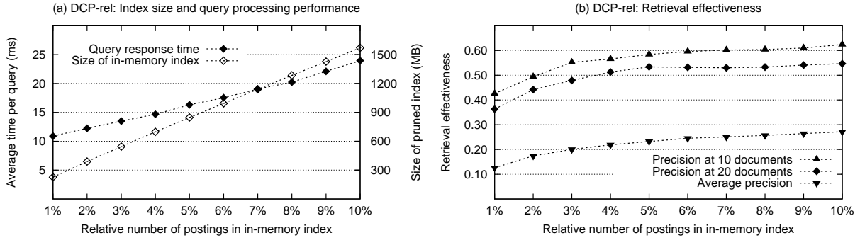
Figure 3: Document-centric pruning with a relative number of postings in the in-memory index ( DCP_{Rel} ). For response times between 11 ms and 24 ms, P@20 varies between 0.3630 ( \lambda = 0.01 ) and 0.5470 ( \lambda = 0.10 ).
