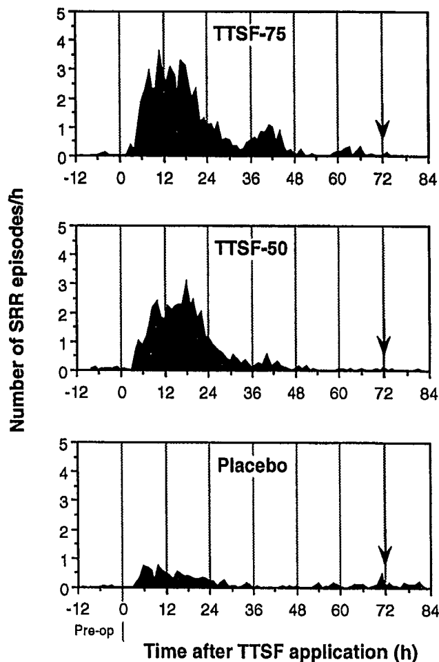
Fig. 4. Mean hourly number of 5-min episodes of slow respiratory rate (SRR, < 8 breaths/min for 5 min). There were significantly more episodes of SRR/h in the TTSF-50 and TTSF-75 groups compared with the placebo group between 5 and 36 h ( P = 0.05 ). The downward-pointing arrow indicates removal of the TTSF patch.
