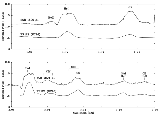
Figure 2. Spectral comparison of #1 from Figer et al. (2005) in the 1806–20 cluster with the galactic dusty WC9 star WR 121 in the H (upper panel) and K (lower panel) band.
