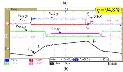
Fig. 15. ZVS performances obtained with (a) conventional SPS and (b) proposed modulation when V_l = 1.4 pu during charging.
