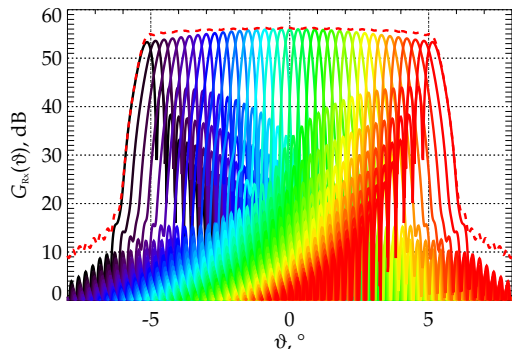
Fig. 7. Co-polar gain patterns for the single-focus reflector with 35 feed elements. The solid lines represent the individual patterns while the dashed line shows the pattern after digital beamforming on receive.
