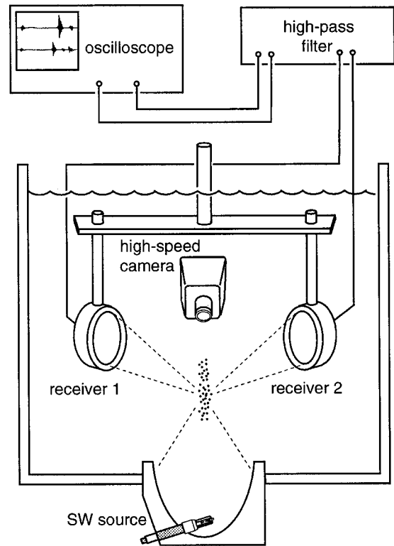
FIG. 5. Setup for high-speed photography and dual PCD.
