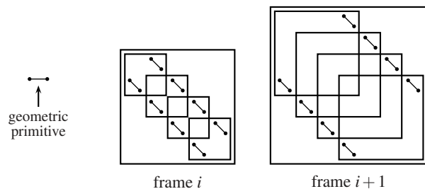
Figure 3: Overlap among children boxes increases because of unstructured relative motion of primitives residing in the same boxes. Note that the severely overlapping child boxes in frame i + 1 will never be used, since the parent will be re-split if encountered during a collision traversal.
