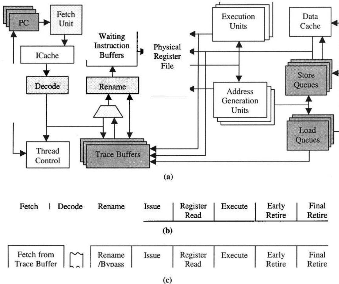
Figure 1: a) DMT block diagram, b) Execution pipeline, and c) Recovery pipeline
