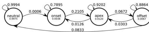
Fig. 12. The states and transition probabilities for an HMM trained on AU 1. Initial probabilities are denoted below the state names. Transitions with probability 0 are not shown.
