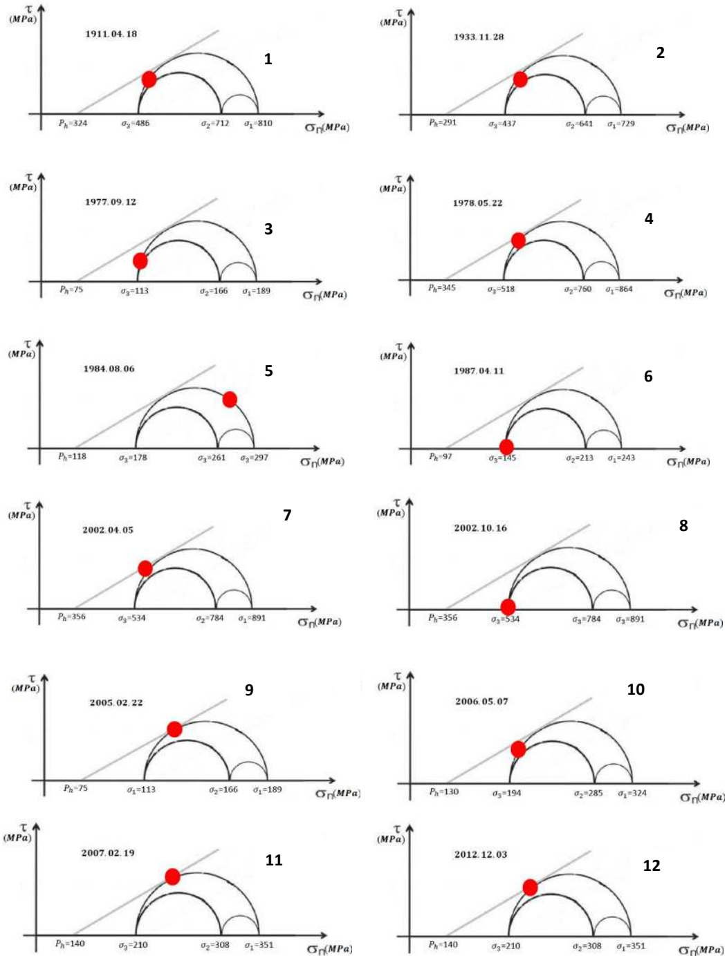
Figure 4. Mohr circles for Kuhbanan fault Earthquakes with a magnitude 5 and more according to Table 1.
