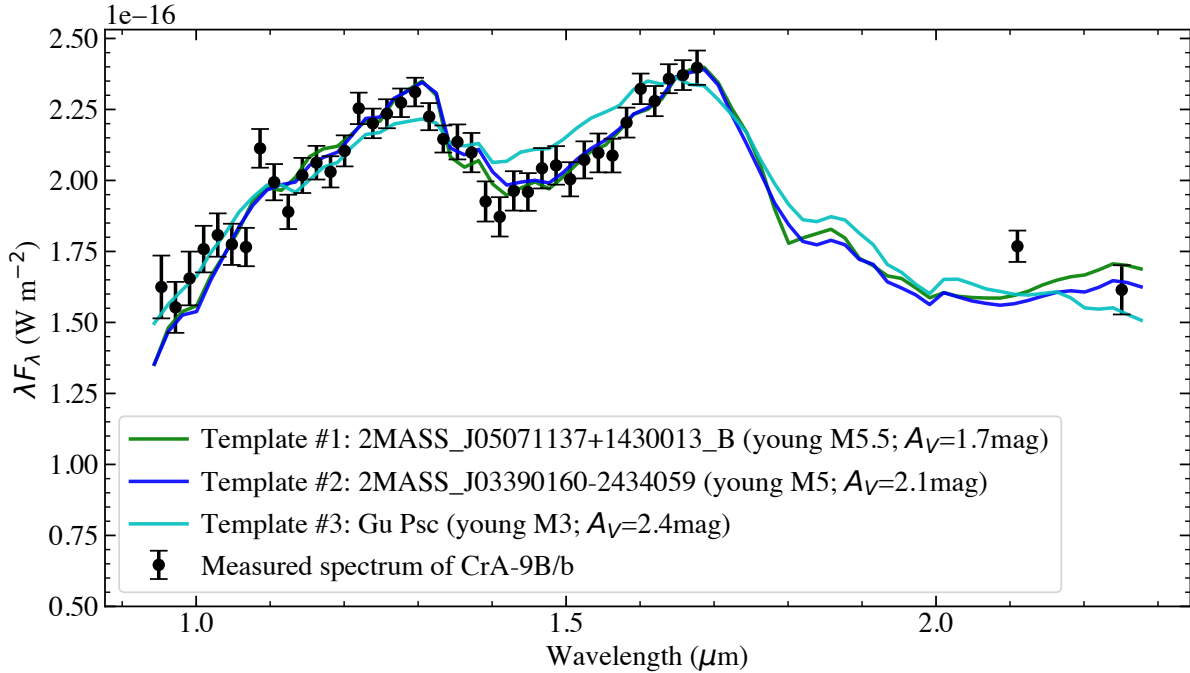
Figure 7. SPHERE (IFS+IRDIS) spectrum of CrA-9 B/b ( black points ) compared to the three best-fit templates of the Montreal Spectral Library: 2MASS J05071137+1430013 B ( \chi_r^2 \sim 1.7 ; Gagné et al. 2015 ), 2MASS J03390160-2434059 ( \chi_r^2 \sim 1.7 ; Gagné et al. 2015 ) and GU Psc A ( \chi_r^2 \sim 1.9 ; Naud et al. 2014 ). The fit considered two free parameters: a scaling factor and optical extinction (whose best-fit value is provided in parenthesis).
