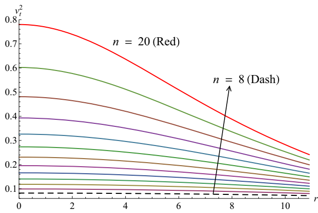
Fig. 7 Variation of v_t^2 ( \text{km}^{-2} ) with radial coordinate r for XTE J1739-285
