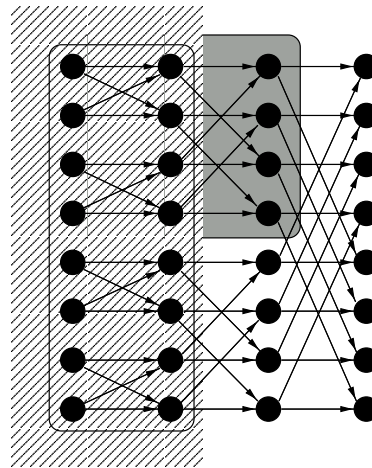
Figure 11: Illustration of the scheduling problem. The butterfly graph (in black) represents an abstraction of the data flow of the fast Fourier transform algorithm on 8 inputs. (In practice, the graph is more complicated because data are complex, and the real and imaginary part interact in nontrivial ways.) The boxes denote two different execution orders that are explained in the text.
