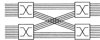
Fig. 3. A 16 \times 16 modified delta network of 8 \times 8 switching elements.
