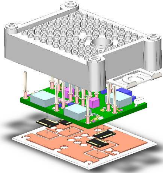
Fig. 3. Three dimensional rendering of the GaN eHEMT power module stack assembly. DBC dimensions are 36x28 mm.
