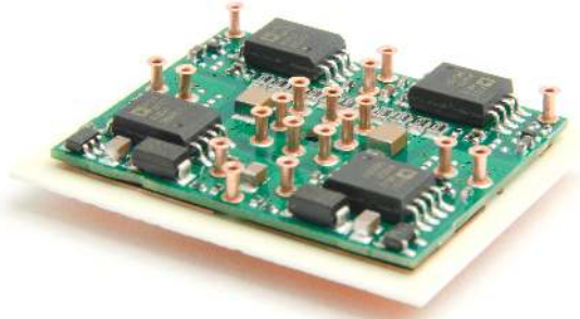
Fig. 13. Photograph of power module after soldering.
