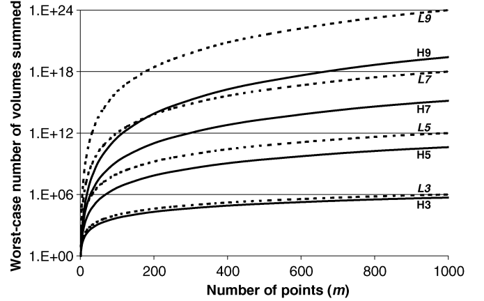
Fig. 7. Log-scale comparison of worst case complexities of HSO and LebMeasure. Each line F_n plots complexity of Algorithm F for m points in n objectives. Solid lines represent HSO and dashed lines represent LebMeasure.
