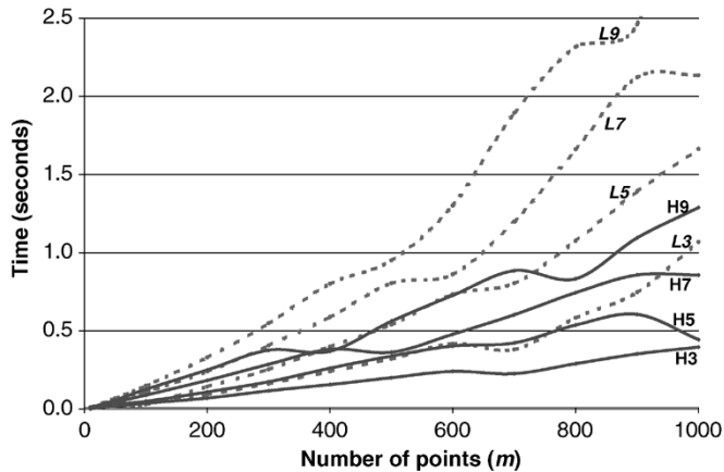
Fig. 14. Comparison of performance of HSO and (optimized) Lebesgue Measure on degenerate front from DTLZ, with objectives in reverse order. Each line F_n plots time taken to run Algorithm F with m points in n objectives. Solid lines represent HSO and dashed lines represent Lebesgue Measure. Each data point is average of ten runs on different data sets.
