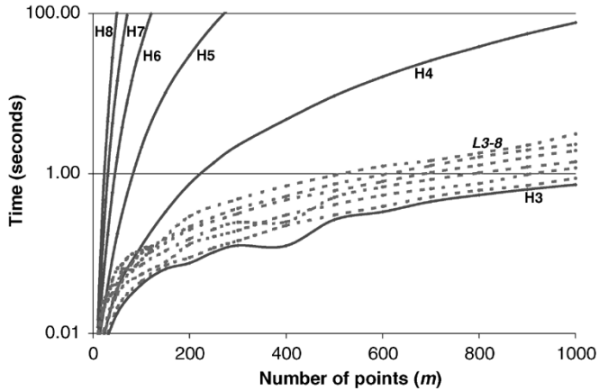
Fig. 12. Log-scale comparison of performance of HSO and (optimized) LebMeasure on degenerate front from DTLZ. Each line F_n plots time taken to run Algorithm F with m points in n objectives. Solid lines represent HSO and dashed lines represent LebMeasure. Each data point is average of ten runs on different data sets.
