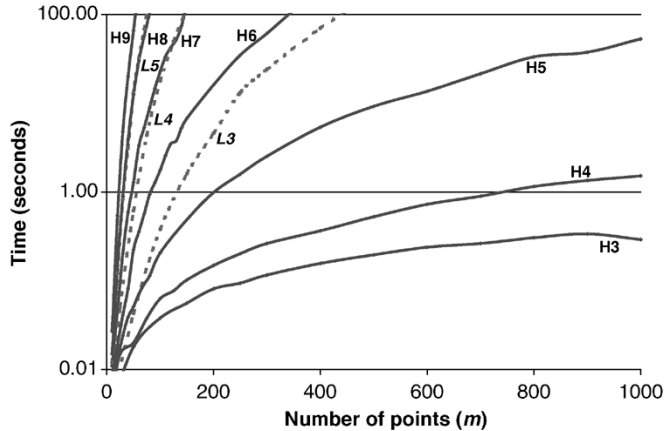
Fig. 8. Log-scale comparison of performance of HSO and (optimized) LebMeasure on randomly generated data. Each line F_n plots the time taken to run Algorithm F with m points in n objectives. Solid lines represent HSO and dashed lines represent LebMeasure. Each data point is average of ten runs on different data sets. L_x coincides with H_{x+3} , 4 \leq x \leq 5 .
