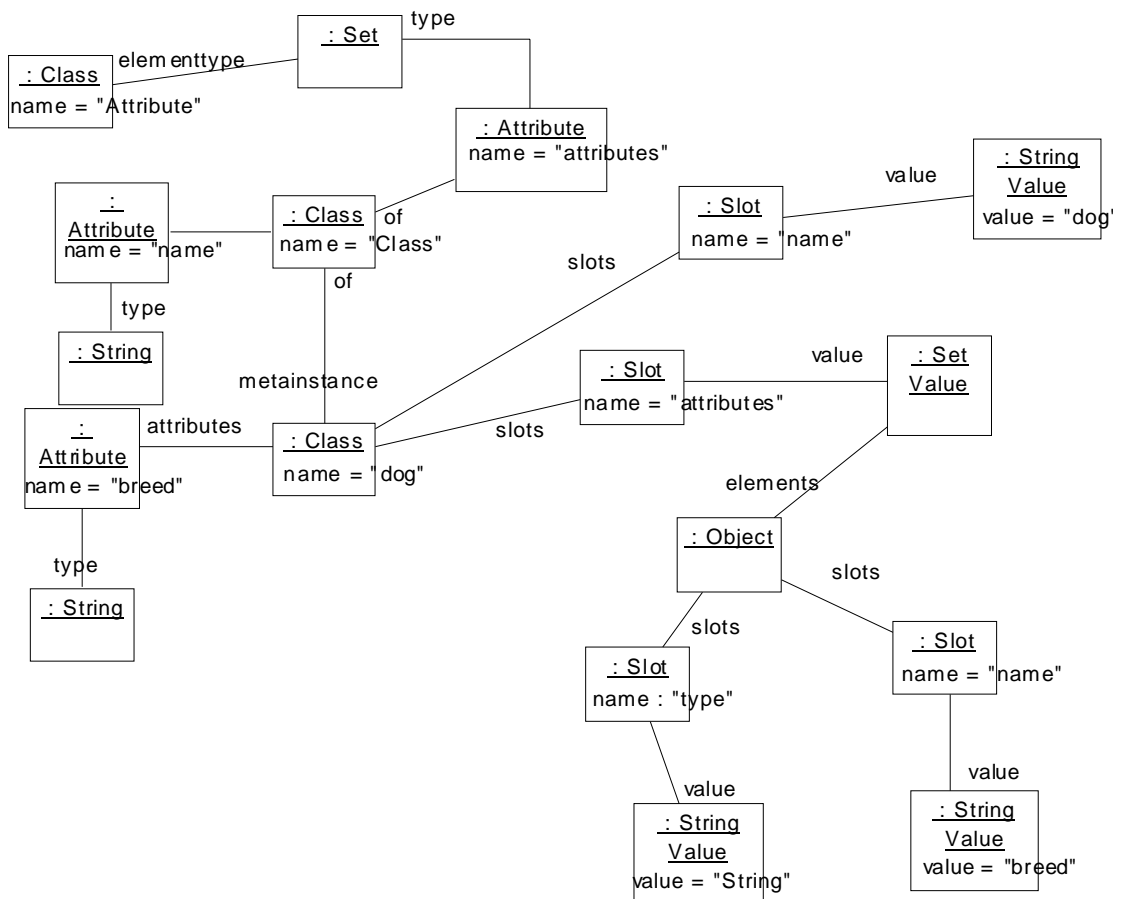
Figure 26. Meta-levels example
