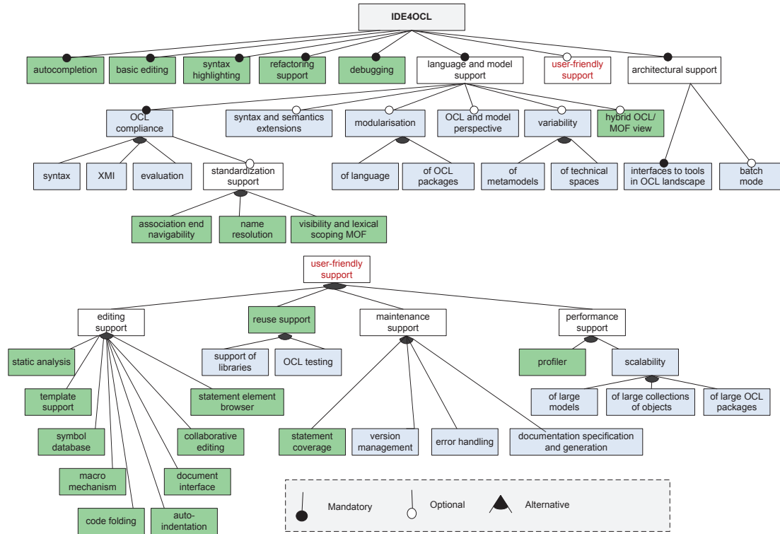
Figure 5: The IDE4OCL feature model with mandatory, alternative and optional features taken from predefined (in green) and proposed (in blue) features.
