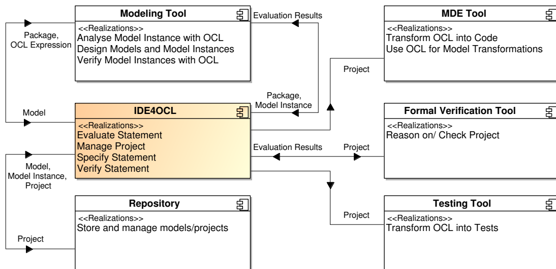
Figure 1: The OCL tools landscape: relations between tools (from [CDSR]).
