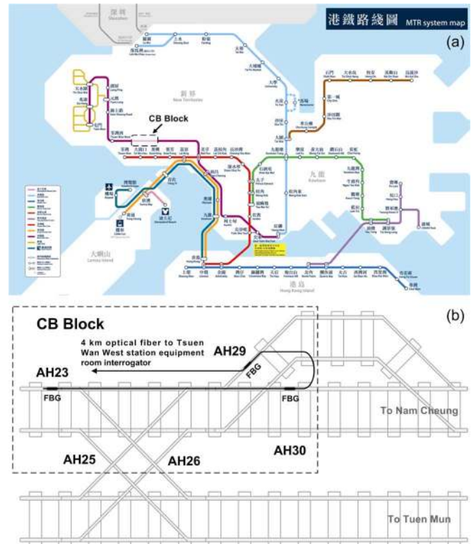
Fig. 5. (a) Route map of the MTR West Rail; the CB block for conducting the test is highlighted. (b) FBG sensors connection in the CB block.
