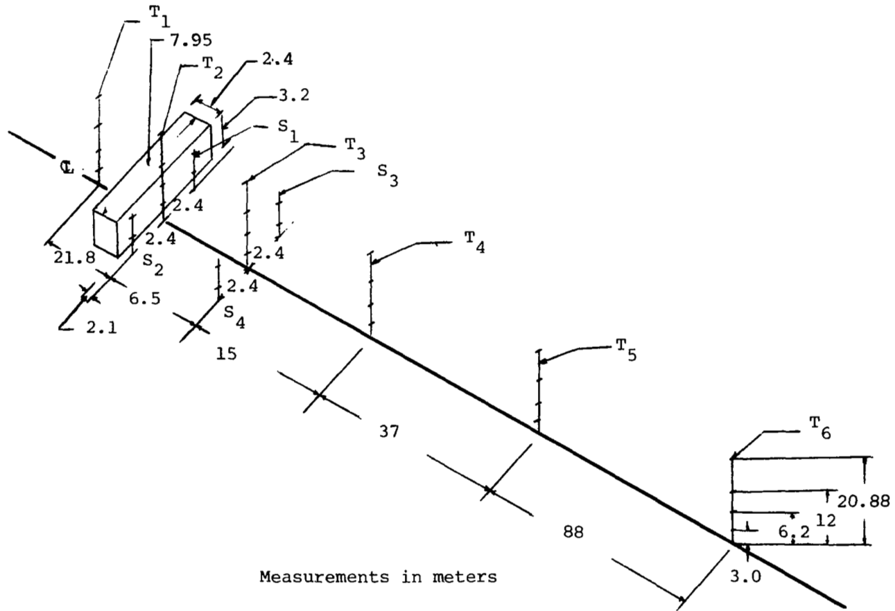
Figure A-3. Tower arrangements; runs 8063 through 8079, recorded between March 1, 1973 and April 27, 1973.
