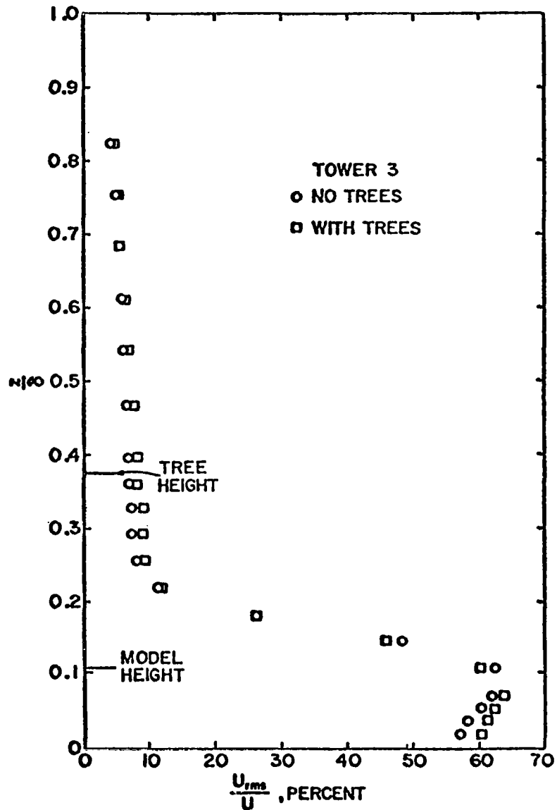
Figure 6. Vertical profile of longitudinal turbulence intensity behind the building model [6].
