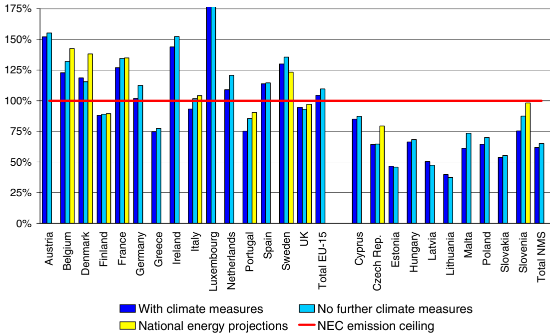
Figure 4.11: Projected NO x emissions for the year 2010 compared with the national emission ceilings
