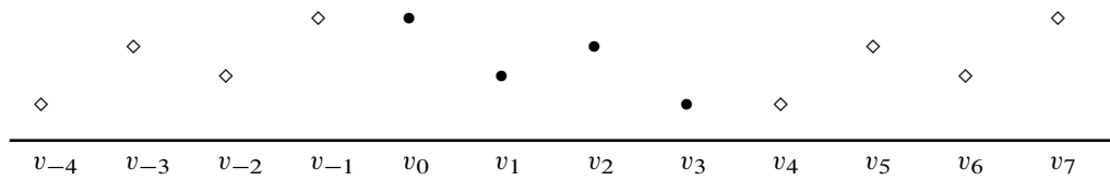
Fig. 2. Entries of the Neumann extension \hat{\mathbf{v}}^{\mathcal{N}} of the vector \mathbf{v} = (v_0, v_1, v_2, v_3) .
