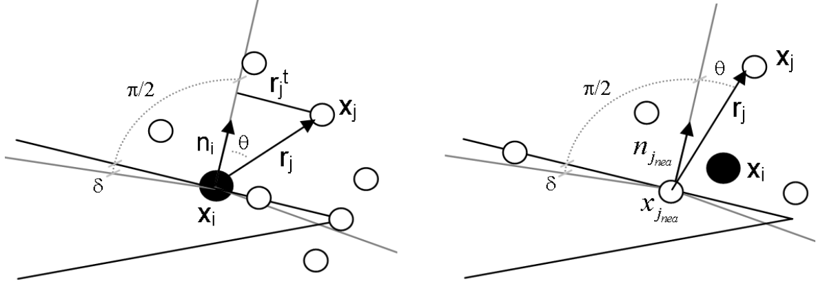
Figure 1: The construction of local clouds near the boundaries. Left: the star point located over a solid boundary; Right: a cloud of points intercepting a solid boundary.
