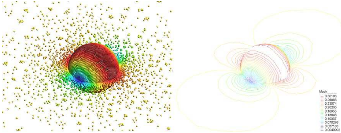
Figure 7: The sphere and the symmetry plane of the problem. Left: points displaying Mach number results; Right: Mach number isolines. M_\infty = 0.2 .
