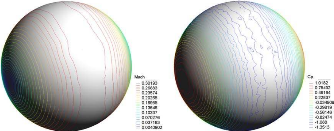
Figure 5: Mach number and C_p isolines on the sphere, M_\infty = 0.2 .
