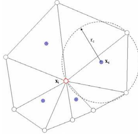
Figure 15: Refinement of a bi-dimensional cloud of points. The filled points x_c meet the requirements r_1 - r_3 and, in consequence, are inserted around the star point x_i .
