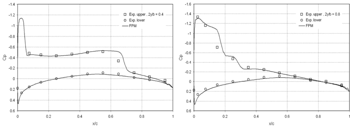
Figure 13: A comparison between computed and experimental C_p distribution along two spanwise wing stations \eta = 0.4 and \eta = 0.8 . NACA wing-body configuration, M_\infty = 0.90 and \alpha = 4.0^\circ .
