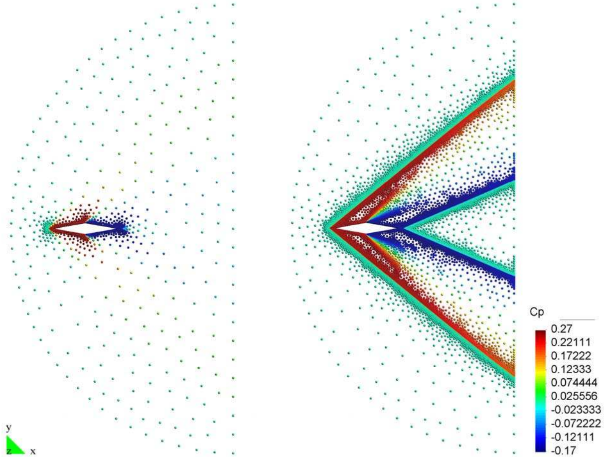
Figure 16: Supersonic flow past a double wedge airfoil. Left: original coarse discretization; Right: final adapted discretization (70 refinement levels). The coloured points show Cp results. M_\infty=2.0 and \alpha=0^\circ .
