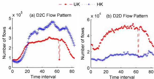
Fig. 6. The D2C and D2D flow patterns during one day in UK and HK.
