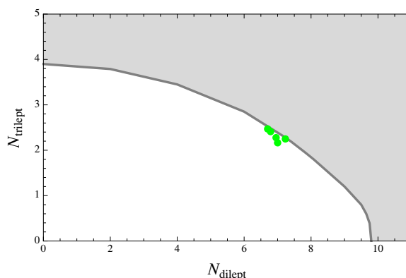
Figure 12. Excluded with 95%CL values of the signal in same-sign dileptons and trileptons channels (gray area) and the maximal allowed values of the di- and trileptons yields according to ref. [50] (green points).
