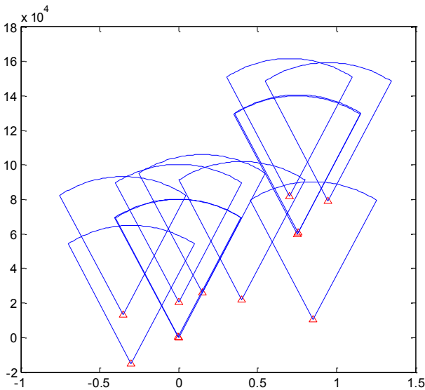
Figure 6. Cooperative detection of formation.
