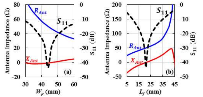
Fig. 6. Simulated antenna impedance, Z_{\text{Ant}} = R_{\text{Ant}} + jX_{\text{Ant}} , and input response S_{11} as function of the patch width W_p , and the length of the microstrip feed line L_f . (a) Variation of W_p with constant L_f = 21 mm. (b) Variation of L_f with constant W_p = 44 mm. The impedance of the antenna is calculated 10 mm from the edge of the patch in the x -axis direction, as shown in Fig. 7.
