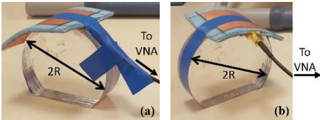
Fig. 15. Experimental setup for E/H bending of the antenna. (a) Bending in the E -plane. (b) Bending in the H -plane.
