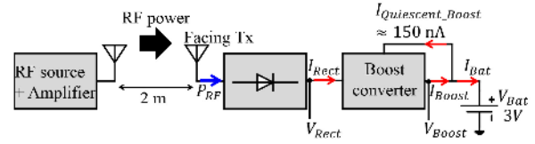
Fig. 25. Experimental setup for the measurement of the complete system. This setup corresponds to one channel where the other channel is identical. For the overall system, the output terminals of the two boost converters are connected in parallel to the output Battery.
