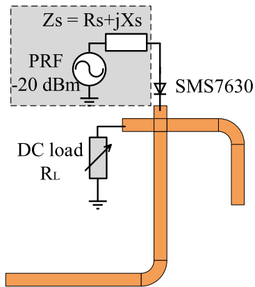
Fig. 10. Harmonic Balance optimization using ADS at -20 dBm input power. For each set of the three variables: R_s , X_s , and R_L , a harmonic balance simulation is run to evaluate the RF/dc efficiency. R_L = 5 k \Omega , R_S = 20 \Omega , and X_S = 260 \Omega are found to maximize the RF/dc efficiency at -20 dBm.
