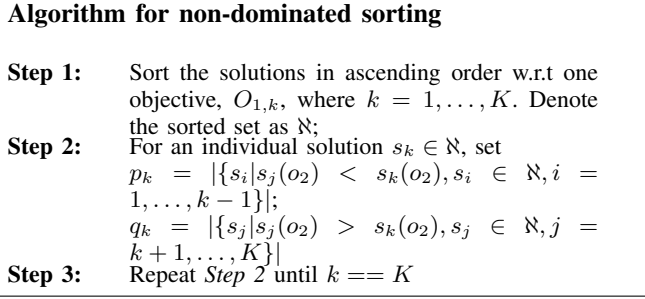
Fig. 5. Algorithm for non-dominated sorting
