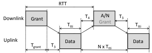
Fig. 2: Uplink round trip time latency budget.
