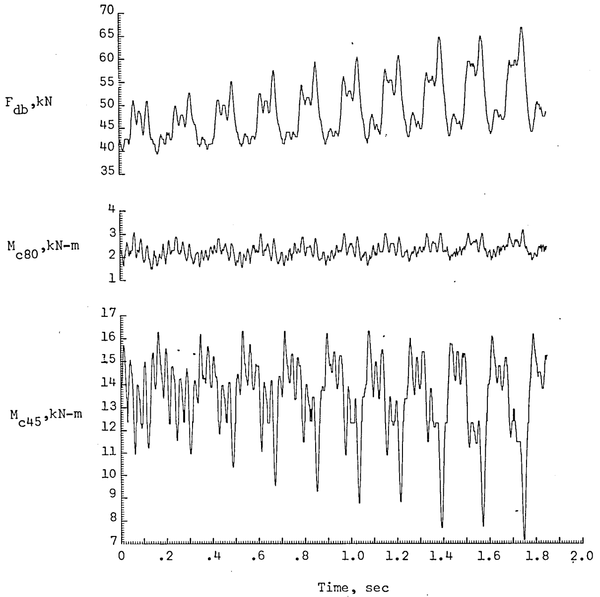
(b) chordwise loads.
