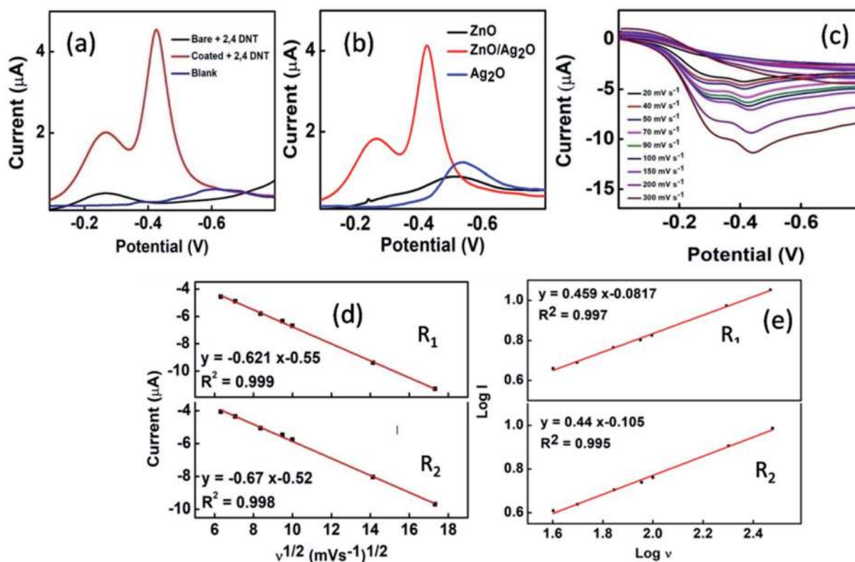
Fig. 3 DPV for (a) bare and a coated electrode for 2,4-DNT ( 20 \mu\text{M} in pH 7, 0.1 mM PBS) and a coated electrode for blank 0.1 mM PBS solution. (b) 2,4-DNT ( 20 \mu\text{M} in pH 7, 0.1 mM PBS) with pure Ag 2 O and ZnO nanoparticles and ZnO–Ag 2 O composite nanoflowers coated electrode. (c) CV for 2,4-DNT ( 20 \mu\text{M} in 0.1 mM, pH 7 PBS) at different scan rates ( 20\text{--}300 \text{ mV s}^{-1} ). (d) Current vs. square root of scan rate ( \nu^{1/2} ) plot. (e) Plot of log current ( I ) vs. log scan rate ( \nu ) for reduction peaks R 1 and R 2 .
