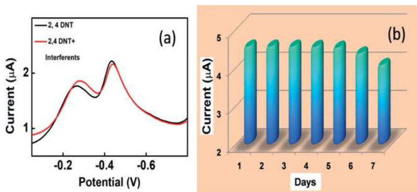
Fig. 6 (a) DPV response for 2,4-DNT (10 \mu\text{M} in 0.1 mM pH 7 PBS) with and without possible interferences. (b) Reusability measurements for 2,4 DNT (20 \mu\text{M} in 0.1 mM pH 7 PBS) for the modified electrode.
