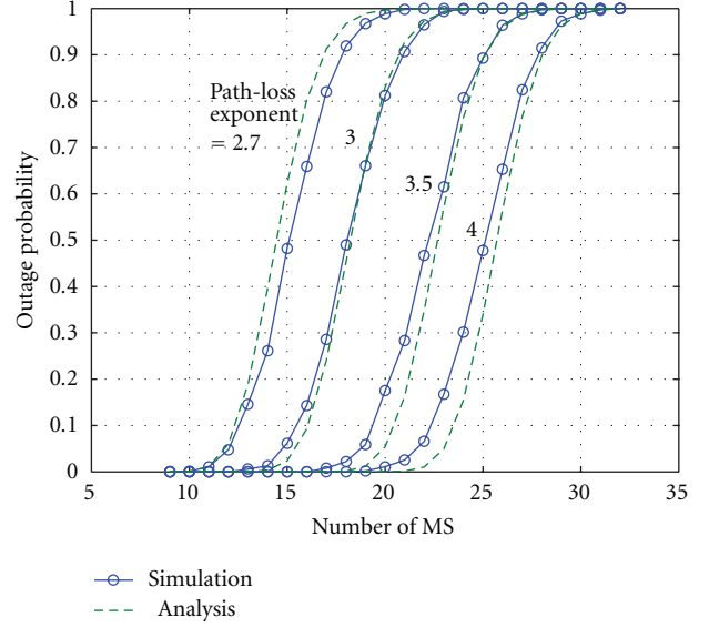
FIGURE 9: Global outage probability as a function of the number of MS per cell and for path-loss exponents \eta = 2.7, 3.5 , and 4 , simulation and analysis.
