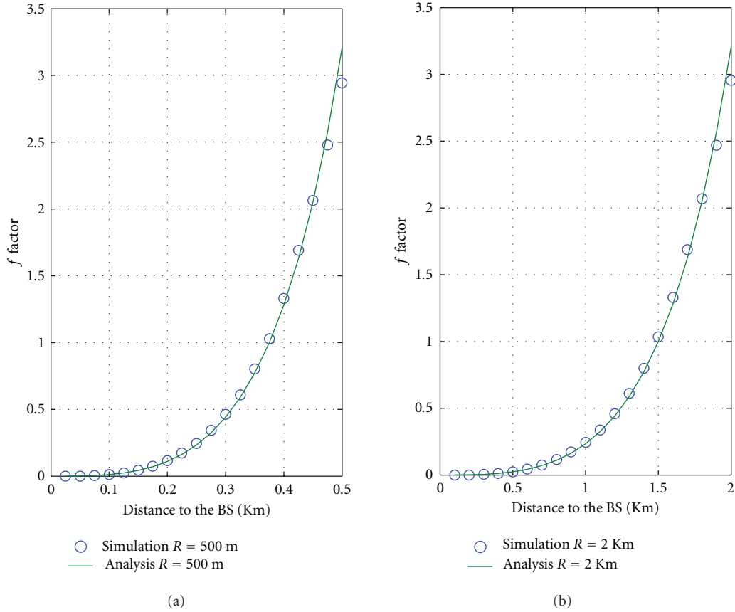
FIGURE 6: OCIF versus distance to the BS; comparison of the fluid model with simulations assuming cell radii R = 500 m and R = 2 Km ( \eta = 3 ).
