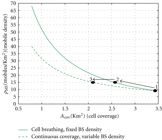
FIGURE 12: Cell breathing (fixed BS density) and BS densification (variable BS density) in a cellular network.
