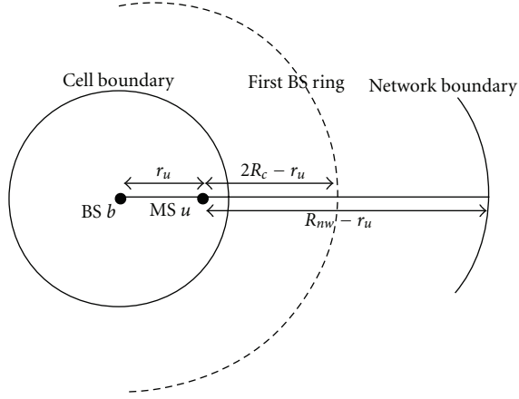
FIGURE 2: Integration limits for external interference computation.
