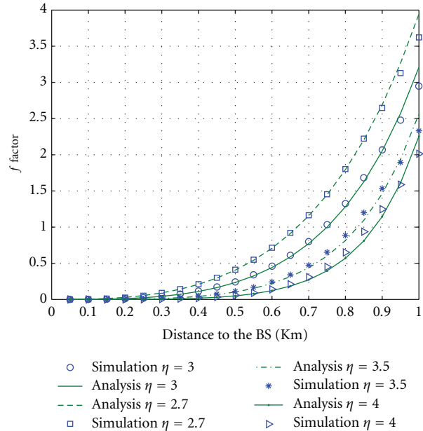
FIGURE 4: OCIF versus distance to the BS; comparison of the fluid model with simulations on a hexagonal network with \eta = 2.7, 3, 3.5 , and 4.
