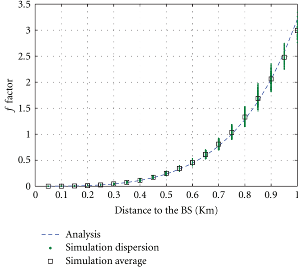
FIGURE 7: OCIF versus distance to the BS; comparison of the fluid model with simulations (average value and dispersion over 500 snapshots) on a hexagonal network with \eta = 3 .
