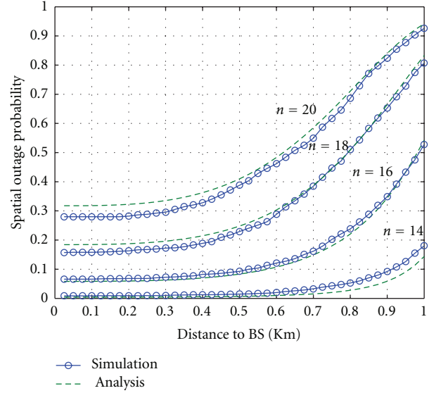
FIGURE 11: Spatial outage probability as a function of the distance to the BS for various numbers of users per cell and for \eta = 3 .
