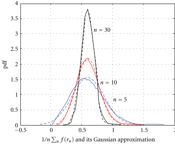
FIGURE 8: Probability density function of (1/n) \sum_u f_u (solid line) and its Gaussian approximation (dotted line).
