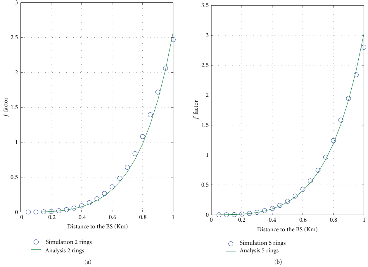
FIGURE 5: OCIF versus distance to the BS; comparison of the fluid model with simulations on a two ring (a) and a five ring (b) hexagonal network ( \eta = 3 ).
