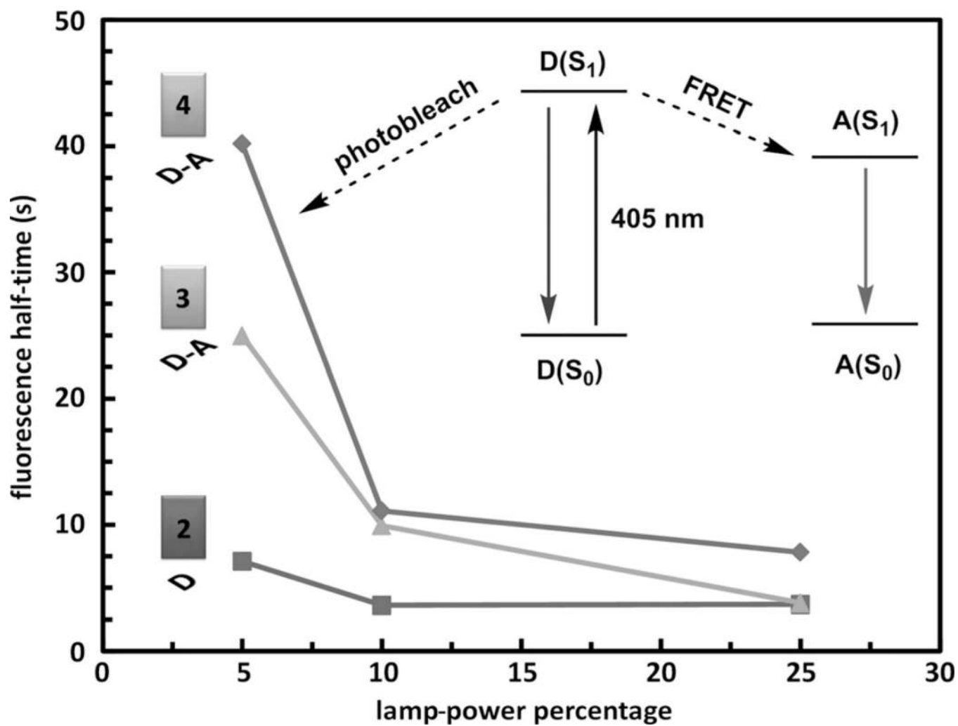
Figure 6. Fluorescence half-time of donor (D) 2 and donor–acceptor conjugates (D–A) 3 and 4 under the zinc(II)-adequate (ZA) conditions as a function of the power of the excitation source (see the Supporting Information for details). Inset: scheme explaining how FRET increases the photostability of the donor (D) component in compounds 3 and 4 .
