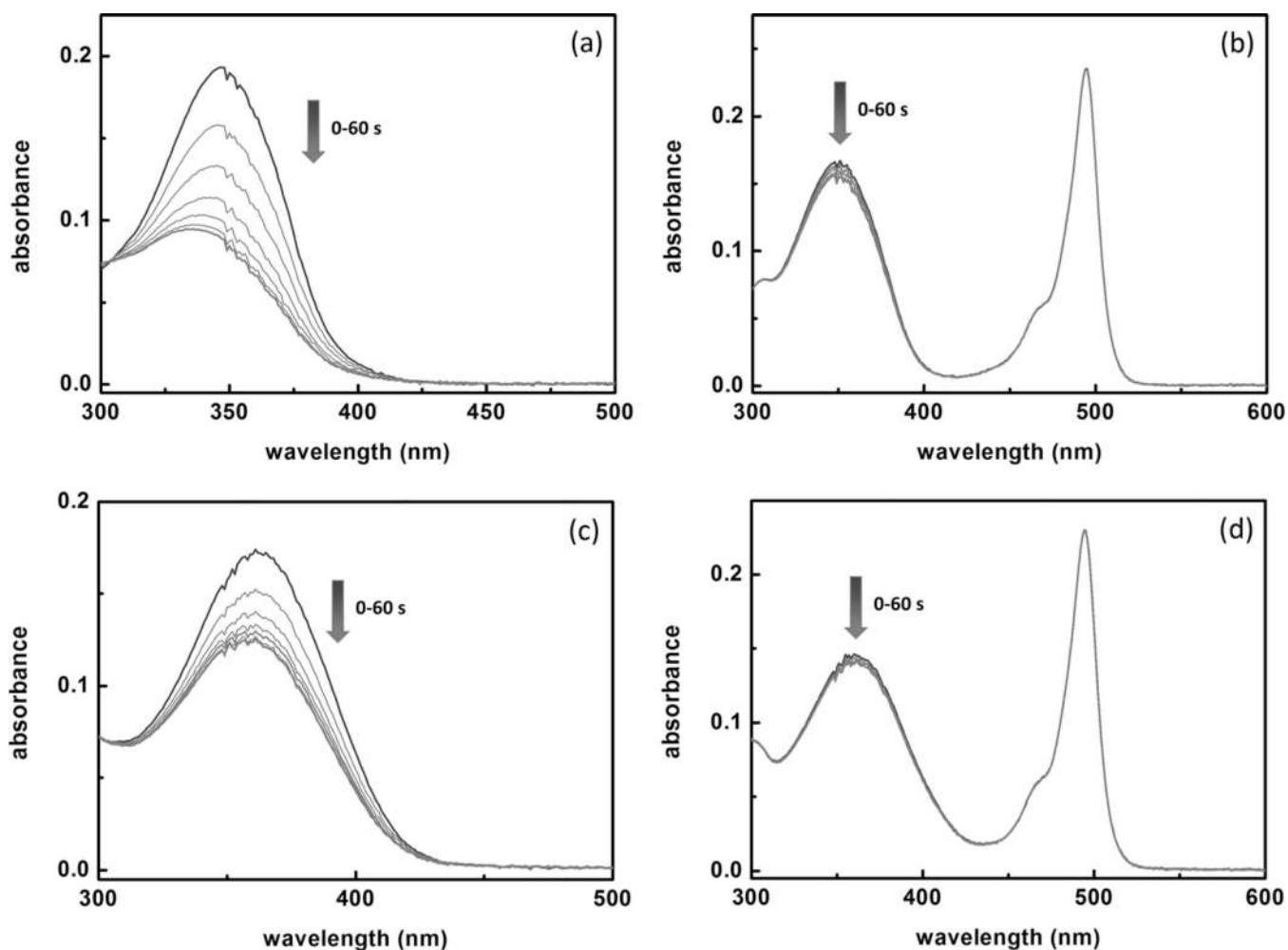
Figure 5. The absorption spectra of compounds a) 2 and b) 4 at 5 \mu\text{M} each in a 1:1 water/ \text{CH}_3\text{CN} mixture at pH 7.3 (HEPES 25 mM, NaCl 25 mM) acquired under irradiation from a handheld UV lamp (365 nm) for 1 min. The spectra were collected at 10 s increments. The changes of absorption spectra of c) 2 and d) 4 under the same conditions in the presence of \text{ZnCl}_2 ( 100 \mu\text{M} ).
