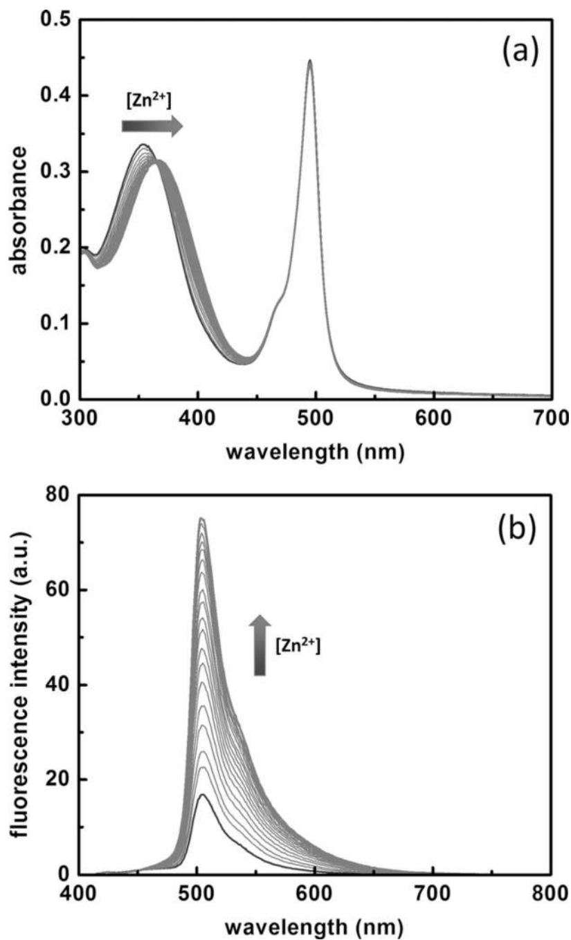
Figure 3. a) Absorption spectral changes of 3 ( 10\ \mu\text{M} ) on addition of \text{ZnCl}_2 (0–12 equiv) in water/ \text{CH}_3\text{CN} mixture (1:1) containing HEPES (25 mM) and NaCl (25 mM) at pH 7.3. b) Corresponding changes in the emission spectra; \lambda_{\text{ex}}=405\ \text{nm} .
