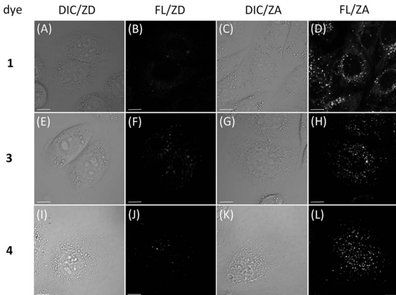
Figure 7. Differential interference contrast (DIC) and fluorescence (FL) images of HeLa (S3) cells incubated with compounds 1 , 3 , or 4 ( 2\ \mu\text{M} , top to bottom) for 30 min, taken under the zinc(II)-deficient (ZD, [\text{ZnCl}_2]=0 ) or the zinc(II)-adequate (ZA, [\text{ZnCl}_2]=50\ \mu\text{M} ) conditions. The growth medium contained sodium pyrithione ( 50\ \mu\text{M} ) as a zinc(II) ionophore. The excitation source was a 405 nm diode laser. The emission window was 500–530 nm. Scale bar = 10\ \mu\text{m} .
